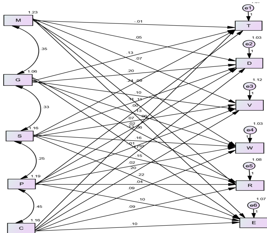
Figure 4.1: Estimated Structural Path Model (AMOS Output)
